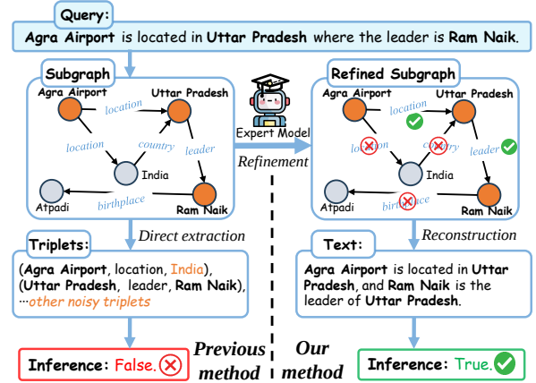
Figure 1: Comparison between previous method and our method. While conventional methods often introduce noisy knowledge during retrieval, our method employs an Expert Model for knowledge refinement, significantly reducing the acquisition of noisy information.
