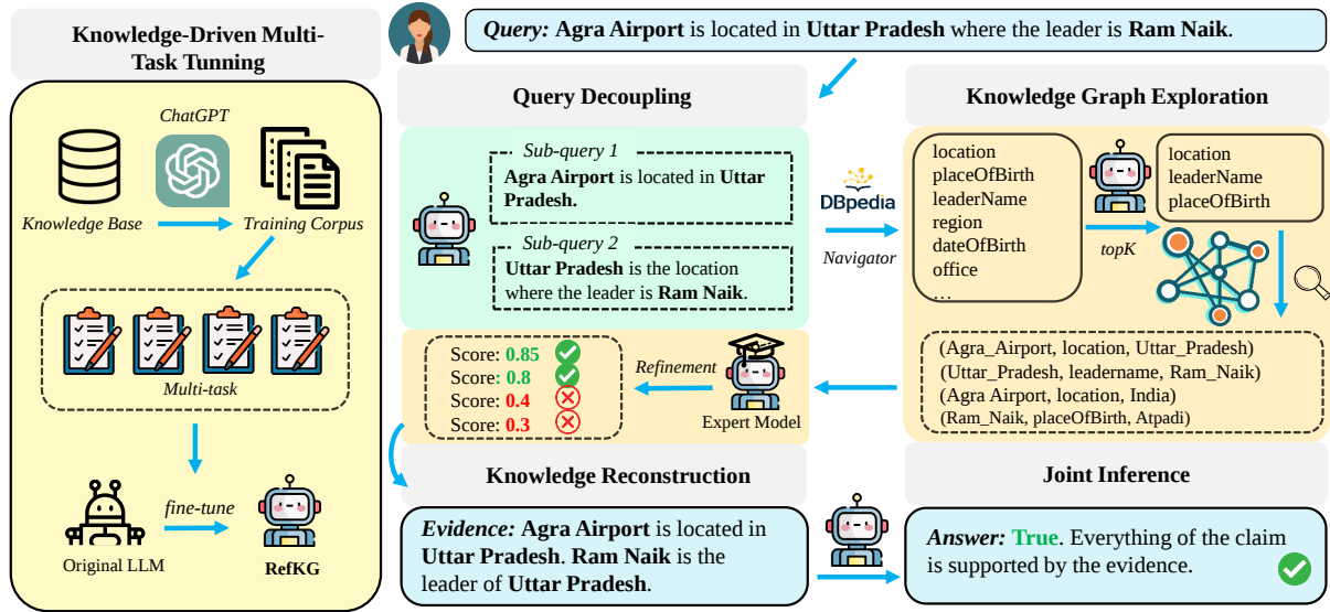
Figure 2: An overview of our proposed framework RefKG. The framework consists of three modules: Query Decoupling , Evidence Subgraph Retrieval and inference with Knowledge Reconstruction . We enhance the model’s ability to utilize knowledge through Knowledge-Driven Multi-Task Tuning, enabling the decoupling, navigation, refinement, and reconstruction of knowledge.
