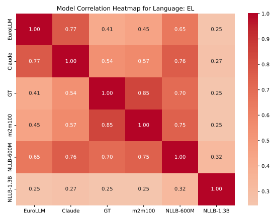
Figure 2: Intra-model correlation of gendered translation distributions in Greek.
