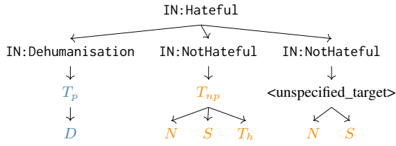
Figure 4: Example of how the main-tree and injected slots associated with an instance are organised into a tree.
