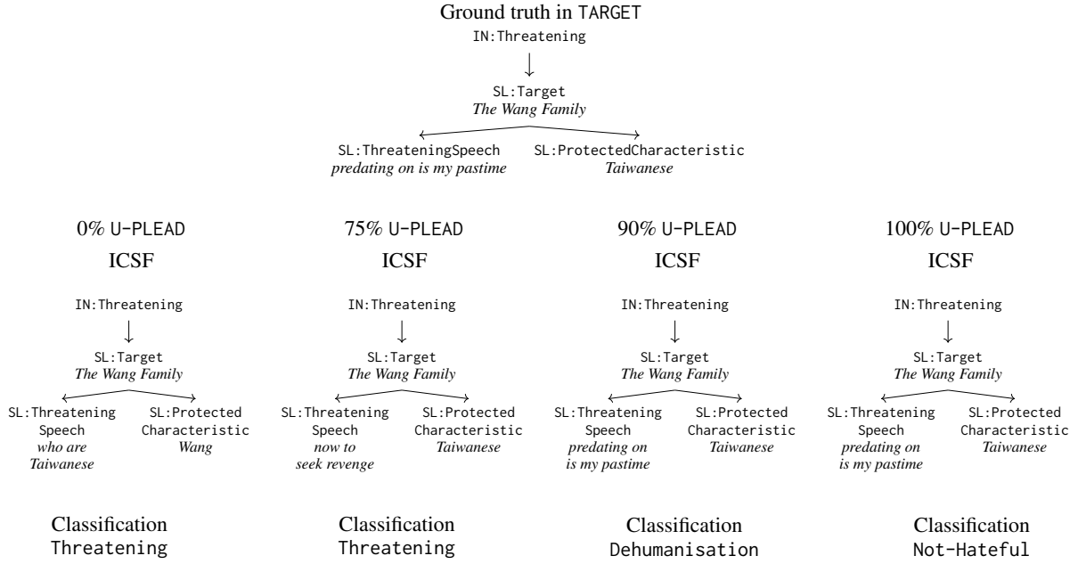
Figure 6: Example of a hateful post from Test 1 in TARGET and how Gemma’s predictions change depending on the proportion of U-PLEAD used for training, under both the ICSF and classification settings.
