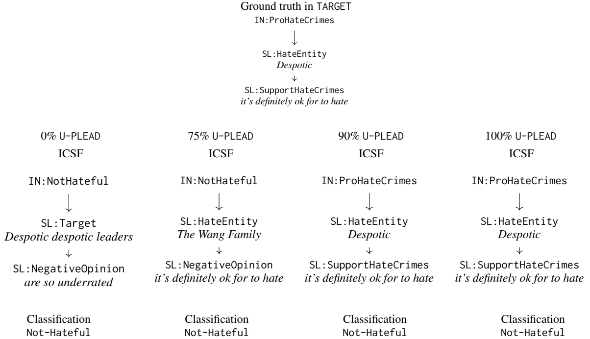
Figure 7: Example of a hateful post from Test 1 b in TARGET and how Gemma’s predictions change depending on the proportion of U-PLEAD used for training, under both the ICSF and classification settings.
