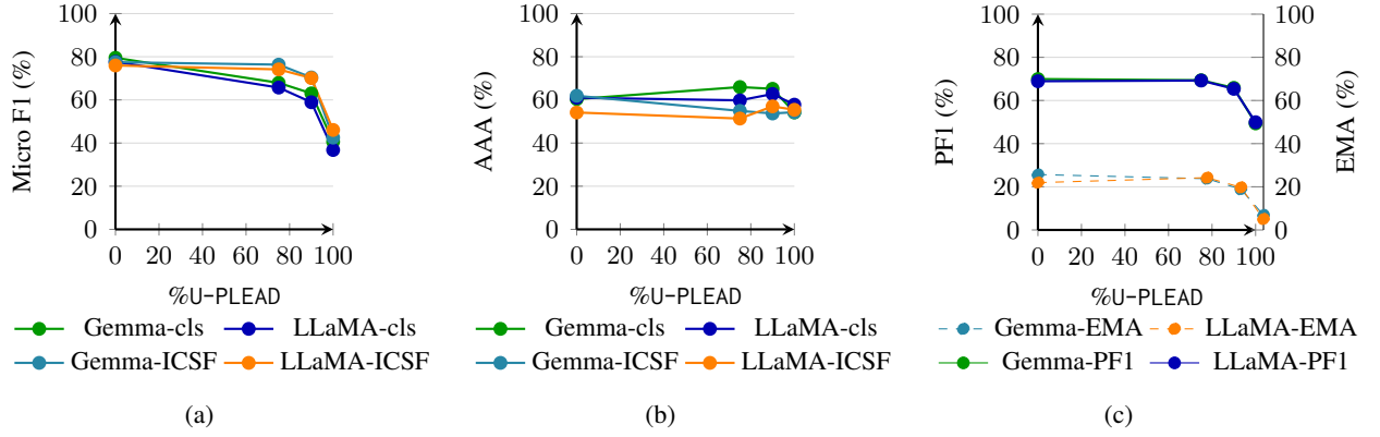
Figure 2: Model performance on intent classification (cls and ICSF settings) using micro F1 (a) and AAA (b). For ICSF models, we also show PF1 and EMA scores (c). Are results are reported on the PLEAD test set.
