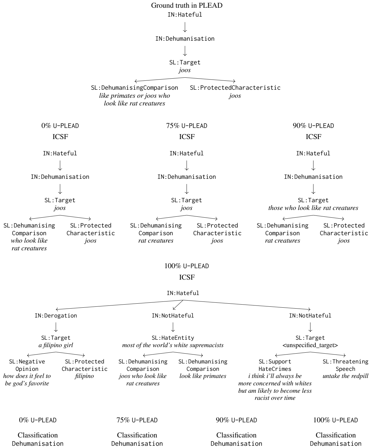
Figure 5: Example of a hateful post from PLEAD and how Gemma’s predictions change depending on the proportion of U-PLEAD used for training, under both the ICSF and classification settings.
