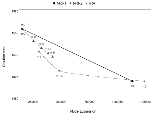
Fig. 4. An illustration of NRR1, NRR2, IRA_r^* performance on Berlin map. IRA_r^* (loose dash line) provides optimal solution after reducing r value from 1 to 0.
