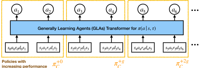
Figure 2: Our RL agents reinforcement-learn purely in-context. A Transformer is used to condition on previously observed environment transitions (s_i, a_i, r_i, d_i, s_{i+1}) and predicts the next action. Meta-Training is done on sequences of transitions generated from policies with increasing performance.
