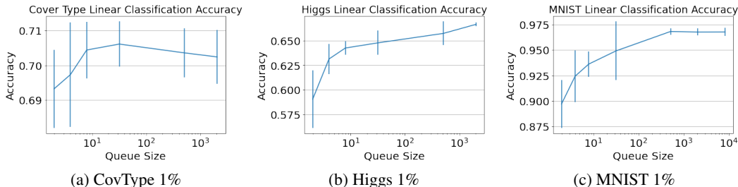
Figure 5: Effect of the queue size on the linear classification accuracy.
