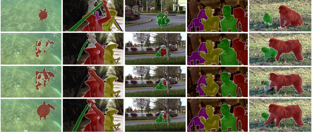
Figure 5. The visualization results on the DAVIS 2019 Challenge. From top to bottom: the first video frame with the ground-truth label followed by results of IRIF [6], CIS [10], and our GIS. The ground-truth of the certain video frame is not publicly available. Our final results significantly track and segment the instances of interest as annotated in the first frame.
