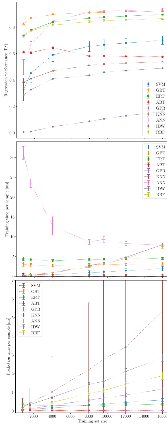
Figure 5. Experiment 3 results, displayed as a function of N_0 . From top to bottom, R^2 , \bar{t}_{\text{trn}} , \bar{t}_{\text{pred}} .
