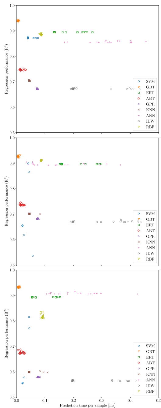
Figure 3. Experiment 1 results. 20 best surrogates per each considered family, plotted in terms of \bar{t}_{\text{pred}} and R^2 with 3 selected slices out of 4 (defined in table 4).
