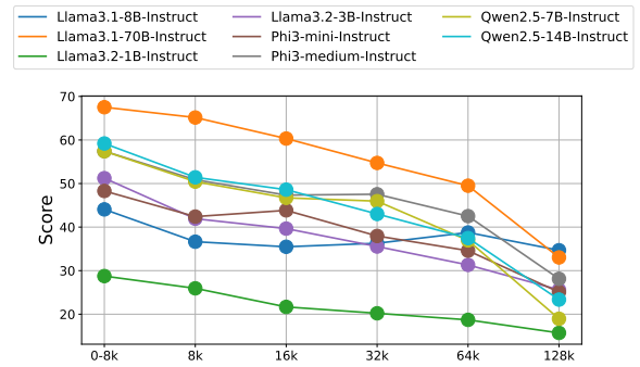
Figure 14: Results of eight open-source models on all tasks in 100 LongBench, showing their scores at different context lengths.
