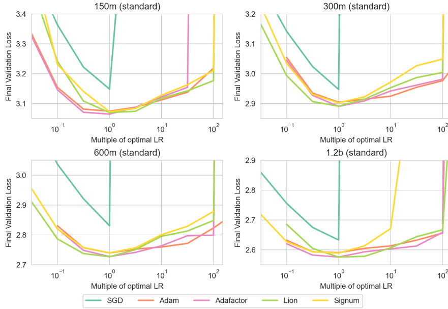
Figure 1: Final validation loss when training language models with 150m, 300m, 600m, and 1.2b parameters, sweeping across learning rates for five standard optimizers (SGD, Adam, Adafactor 1 , Lion, and Signum). Plots have been shifted to align the optimal learning rates for each optimizer. Except for SGD, other optimizers seem comparable in their optimal performance and stability with respect to learning rate tuning.
