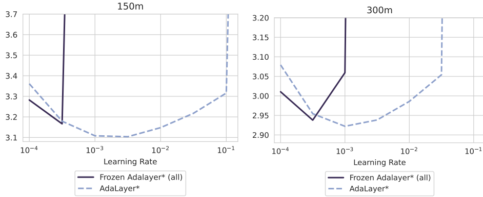
Figure 17: Training 150m ( Left ) and 300m ( Right ) models using fixed Adalayer* learning rate ratios from initialization for all layers. We observe this quickly diverges, achieving neither peak performance nor stability.
