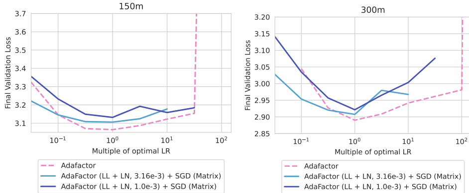
Figure 14: Training 150m ( Left ) and 300m ( Right ) models using Adafactor on the last layer with a fixed learning rate and using SGD on other matrix blocks. We see that performance and stability is comparable to Adafactor, but does not exceed it, particularly at higher learning rates.
