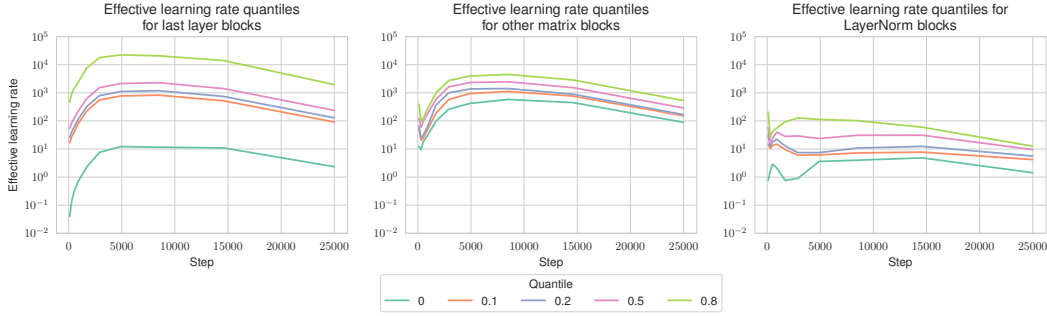
Figure 7: Quantiles of effective learning rates ( \eta_t/(\sqrt{v_t} + \epsilon) for each layer l ) for the last layer blocks ( Left ), the LayerNorm blocks ( Right ), and the other matrix blocks ( Middle ) for a 150m model trained using Adalayer*. Unlike the other matrix blocks and LayerNorm parameters, the effective learning rates across logits vary across multiple orders of magnitude, providing evidence for the need to precondition them separately.
