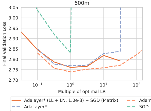
Figure 11: As in Section 3.2, we train 300m ( Left ) and 600m models ( Right ) with Adalayer* on the last layer and LayerNorm parameters, and train the remaining model parameters with SGD. We see that performance and stability continues to match that of Adalayer* or outperform Adalayer* even at these larger scales..
