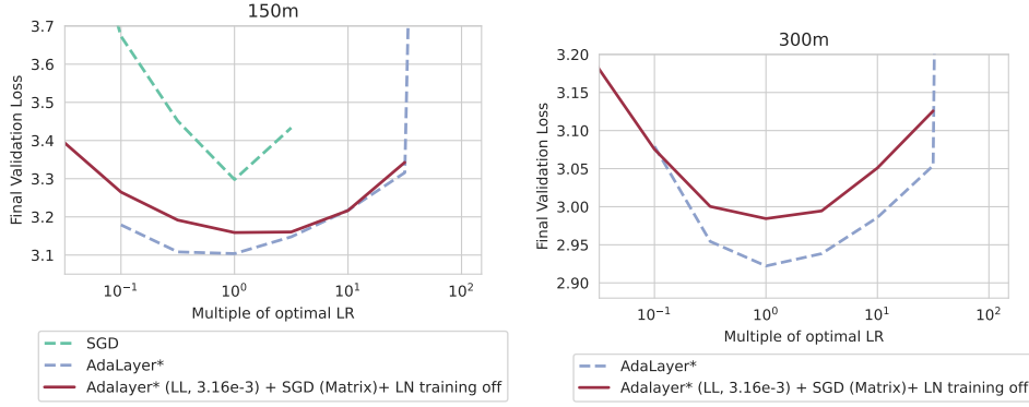
Figure 13: Training 150m ( Left ) and 300m ( Right ) models using Adalayer* on the last layer with a fixed learning rate of 3.16e-3 and using SGD on other matrix blocks, while turning off the option to train LayerNorm parameters. We see that while the performance and stability is improved compared to SGD, it is still not as performant as Adalayer*. This indicates a degree of importance of training LayerNorm parameters for these models.
