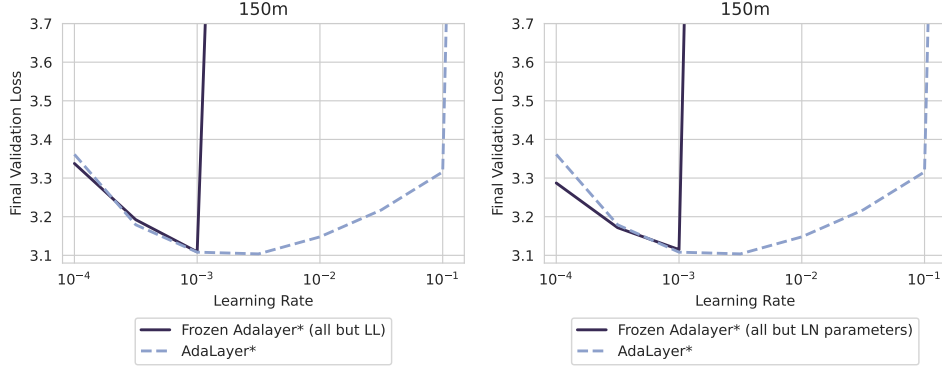
Figure 18: Training 150m models using fixed Adalayer* learning rate ratios from initialization while either excluding only the last layer ( Left ) or excluding only the LayerNorm parameters ( Right ). We observe both modifications reach peak performance but fails to be stable at higher learning rates.
