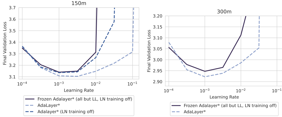
Figure 19: Training 150m ( Left ) and 300m ( Right ) models using fixed Adalayer* learning rate ratios from initialization, while letting the last layer continue to update, and turning LayerNorm training off. Stability across learning rates has improved but is less performant; for the 150m model we also plot the sweep for regular Adalayer* with LayerNorm training off, and we see that it is worse in performance compared to Adalayer* with LayerNorm training.
