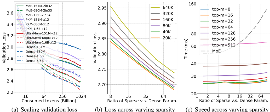
Figure 6: (a). C4 validation loss of different models at different scale. (b). Scaling curves at different sparsity with 151M activated parameters. Each line represents the same model sparsity; e.g., 20K indicates that approximately one out of every 20,000 values will be activated. The loss decreases linearly as the sparse parameters increase exponentially. (c). Inference time for UltraMem and MoE with 1.6B activated parameters. The batch size is 512, sequence length is 1, and key/value cache length is 2048. With fixed activation parameters, UltraMem’s inference time remains nearly constant as sparse parameters increase, while MoE’s inference time increases significantly.
