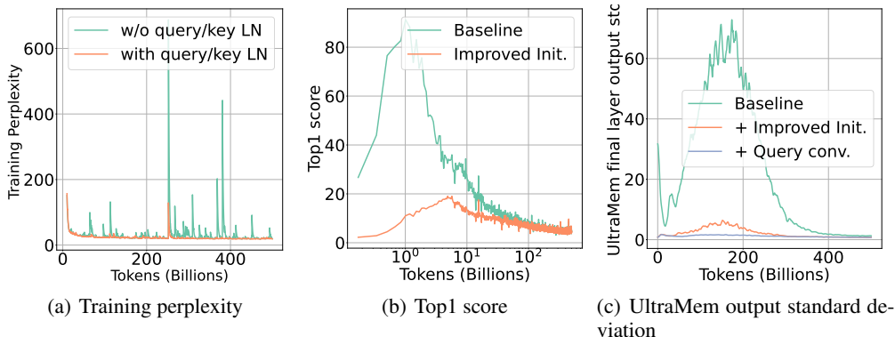
Figure 10: Model training state details. “Top1 Score” refers to the highest score among the retrieved keys. “UltraMem Output Std” represents the standard deviation of the outputs from the last layer of UltraMem.
