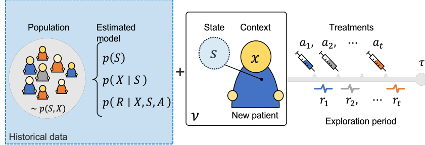
Figure 1: Illustration of the pure-exploration latent bandit problem and the example of treatment personalization. A population of patients have been observed in historical data to learn the distribution of latent states P(S) , P(X|S) and the conditional reward the distribution P(R|X, S, A) . A new patient, represented by the instance \nu = (x, s) is treated with actions a_t , observing rewards r_t until the stopping time \tau .
