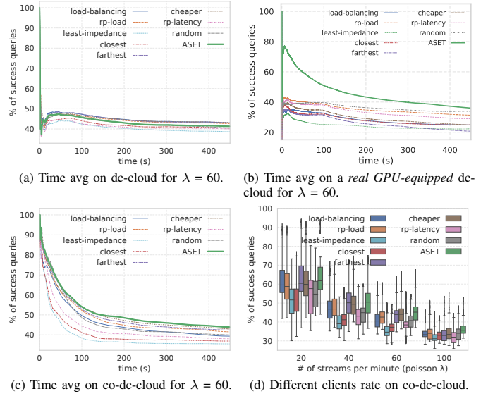
Fig. 5: Performance of ASET compared to static policies for the dc-cloud topology on (a) simulated and (b) real-deployment scenario, and (cd) the co-dc-cloud topology.
