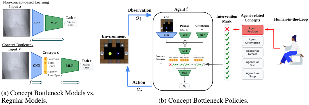
Figure 1: Concept bottleneck models force neural network classifiers to make decisions through an intermediate set of human-understandable concepts. Concept Bottleneck Policies increase the interpretability of emergent multi-agent behavior in a similar manner—distilling agent strategies into concepts—yielding interpretable, concept-based policies for MARL. CBPs also enable post-hoc behavioral analysis via concept intervention, which reveals the inter-agent factors driving coordination.
