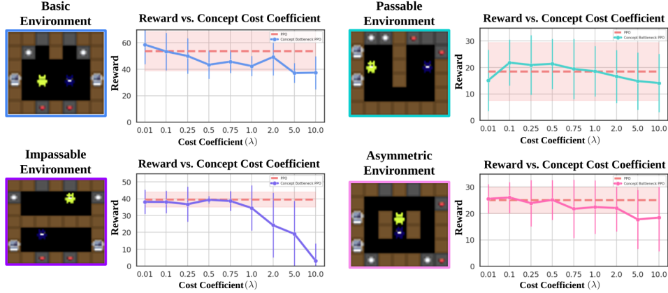
Figure 5: Performance of ConceptPPO and PPO in the cooking domains. With \lambda \leq 0.5 , ConceptPPO matches the performance of non-concept-based PPO. This indicates that ConceptPPO achieves interpretability without sacrificing performance. For higher values of \lambda , agent behavior changes as a result of over-valuing the concept prediction loss, which in turn impacts performance.
