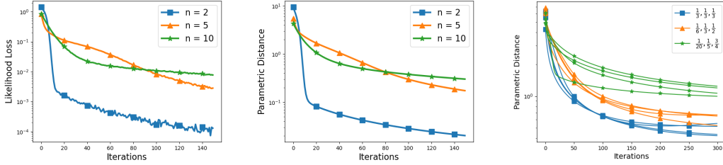
Figure 1: Left: Sublinear convergence of the likelihood loss \mathcal{L} . Middle: Sublinear convergence of the parametric distance \sum_{i \in [n]} \pi_i \|\mu_i - \mu^*\|^2 between student GMM and the ground truth. Right: Impact of different mixing weights on the convergence speed.
