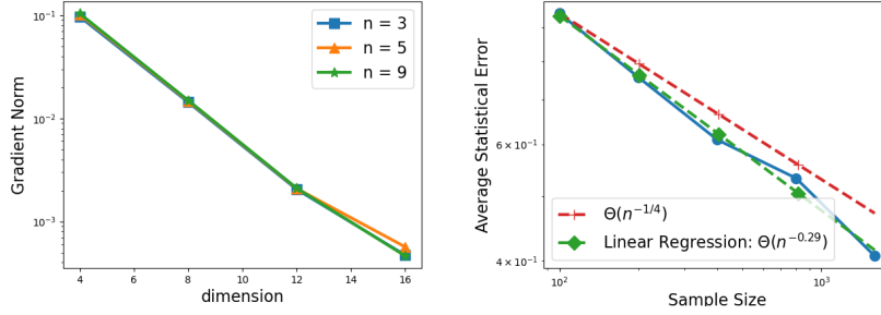
Figure 2: Left: Gradient norm \|\nabla \mathcal{L}(\mu(0))\| in the counter-example in Theorem 7 decreases exponentially fast w.r.t. dimension d . Right: The statistical error (blue line) approximately scales as \sim n^{-1/4} with sample size n .
