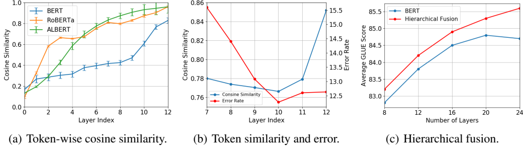
Figure 1: Over-smoothing in BERT models.
