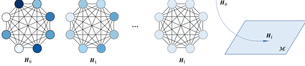
Figure 4: The illustration of over-smoothing problem. Recursively, \mathbf{H}_l will converge to subspace \mathcal{M} where representation of each token is identical.
