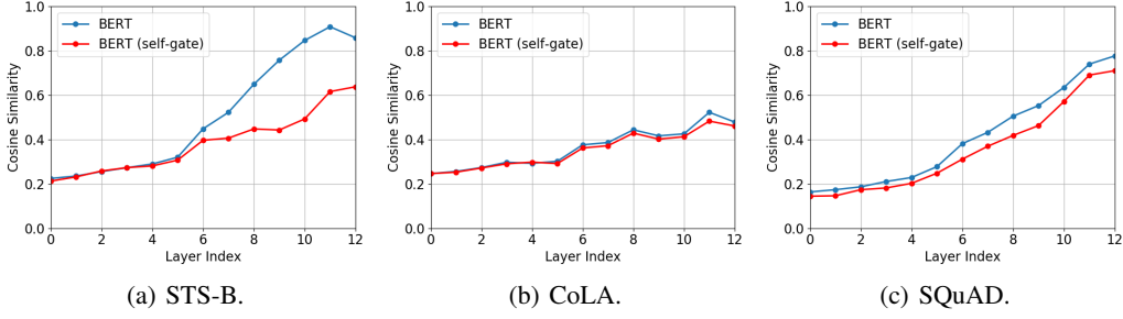
Figure 6: The token-wise similarity comparison between BERT and BERT with self-gate fusion.
