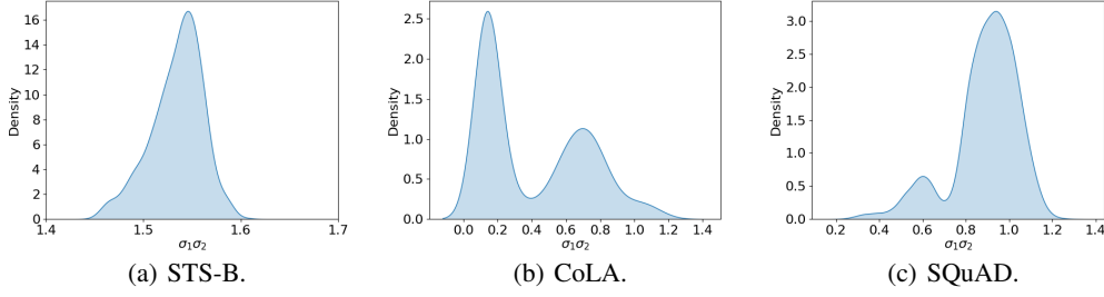
Figure 5: The estimated distribution of \sigma_1\sigma_2 for different fine-tuned models.
