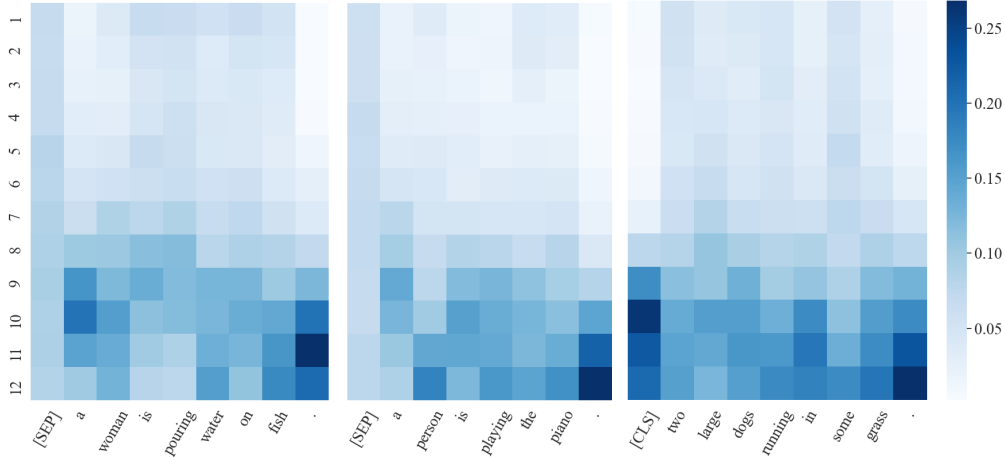
Figure 7: Visualization of importance weights of self-gate fusion on different layers.
