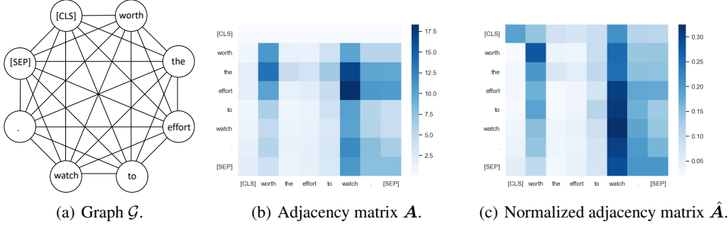
Figure 2: Illustration of self-attention and the corresponding graph \mathcal{G} . For simplicity, we drop the self-loops in \mathcal{G} .
