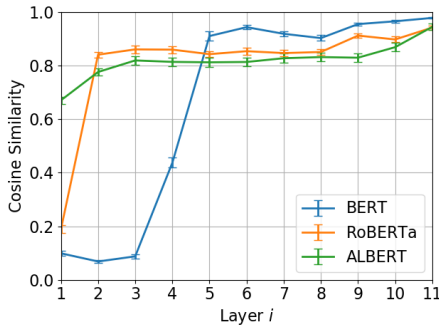
Figure 3: Cosine similarity between the attention matrices \hat{\mathbf{A}} 's at layer i and its next higher layer.
