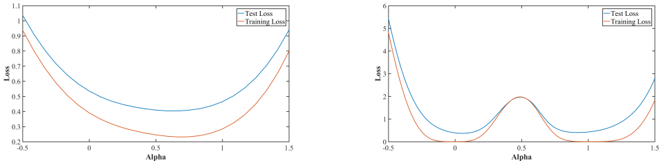
(a) Training and test loss for interpolations between two network states from regular ResNet training. (b) Training and test loss for interpolations between two CLR “solutions.”
