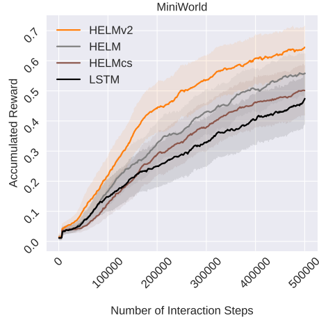
Figure 3: IQM and 95% bootstrapped CIs across 30 seeds for 6 MiniGrid environments ( left ), and 8 more 3D MiniWorld environments ( right ).
