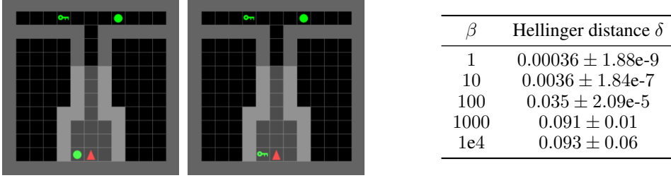
Figure 1: Left: Instances of the MiniGrid-Memory environment. The agent only observes the white shaded region, and must navigate to the object seen in the starting room. Right: Hellinger distance (Hellinger, 1909) of softmax distributions over token embeddings for the two observations of the Memory environment depicted on the left. Mean over 1000 different initializations of \mathbf{P} of FH is shown. For very high values of \beta > 1\text{e}4 , the softmax converges to a one-hot encoding and \delta directly corresponds to the probability of mapping to a single, but different token embedding. Therefore, with higher values of \beta , there is only a \sim 10\% chance of avoiding collapse to the same token embedding.
