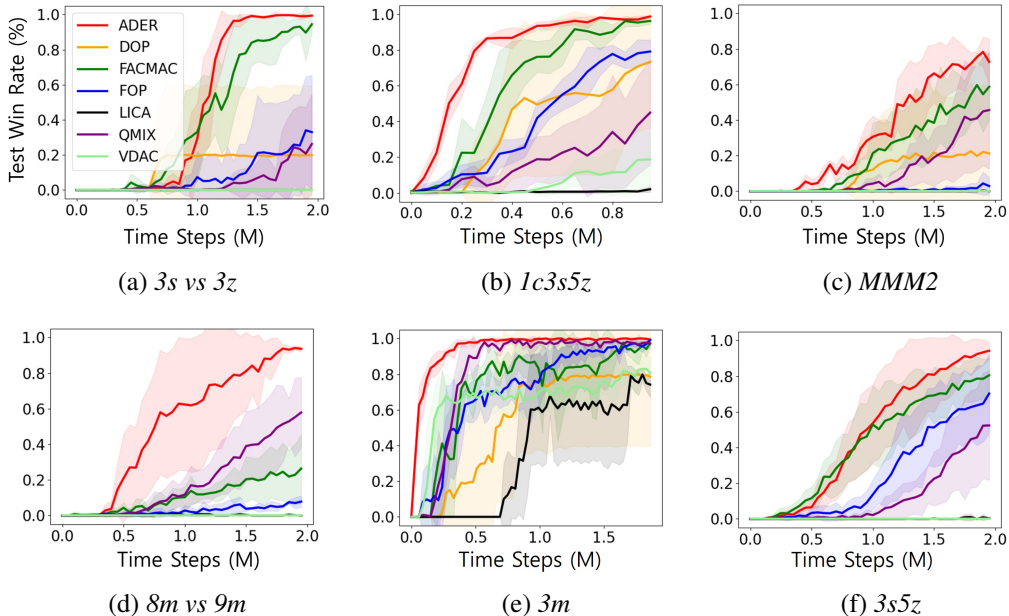
Figure 8: Average test win rate on the SMAC maps.
