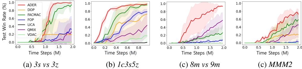
Figure 4: Average test win rate on the SMAC maps. More results are provided in Appendix D.
