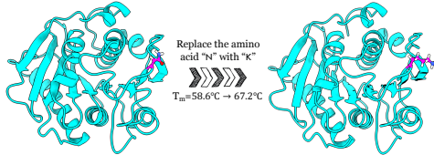
Figure 4: Visualization of an AI design that thermostabilized a protein. The amino acid “N” was predicted by the MutCompute web server to be mutated to a “K”, which was experimentally shown to improve thermostability by 8.6°C and was critical for the engineering of FAST-PETase (Lu et al., 2022). ThermoPETase structure (left) (PDB: 6ij6) and the mutated one (right) was obtained via (Waterhouse et al., 2018).
