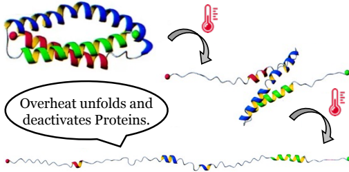
Figure 1: Overheat unfolds and deactivates proteins (Paci & Karplus, 2000).
