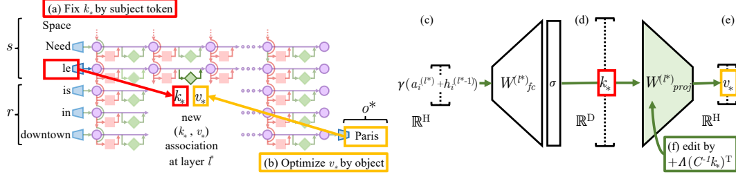
Figure 4: Altering weights of a single MLP layer with ROME. To associate the Space Needle with downtown Paris , the ROME method inserts a new (k_*, v_*) association into layer l^* , where (a) the key k_* is determined by the subject and (b) the value v_* is optimized to select the object. (c) Hidden state at layer l^* and token i passes through the MLP’s fc matrix to produce (d) the key vector k_* that identifies the subject. (e) To write new value vector v_* into the layer, (f) we calculate a rank-one update \Lambda(C^{-1}k_*)^T for the proj matrix to cause \hat{W}_{proj}^{(l*)}k_* = v_* while minimizing interference with other memories stored in the layer.
