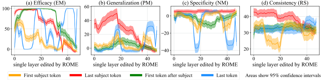
Figure 5: ROME edits are benchmarked at each layer-and-token combination in GPT-2-XL. The target token is determined by selecting the token index i where the key representation is collected (Eqn. 3). ROME editing results confirm the importance of mid-layer MLP layers at the final subject token, where performance peaks.
