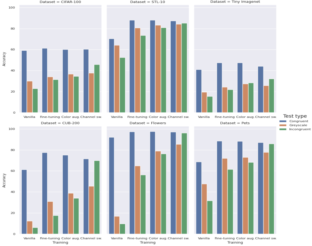
Figure 3: Top-1 \mathcal{D}^{test} accuracies for different training strategies.
