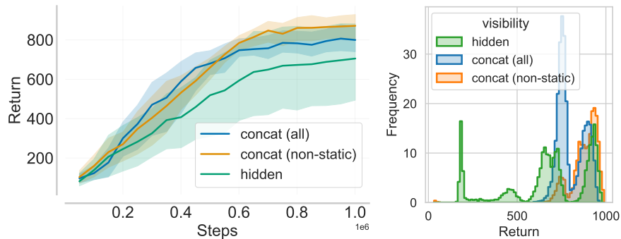
Figure 2: Train (lineplot) and test performance (histogram) of agents with visible and hidden context on CARLdmcWalker with different viscosity values and 5 seeds. Shown is the mean performance with a 95% confidence interval and testing across 200 test contexts (metrics are computed using stratified resampled bootstrapping [3]). Here, concatenating context to the state seems beneficial.
