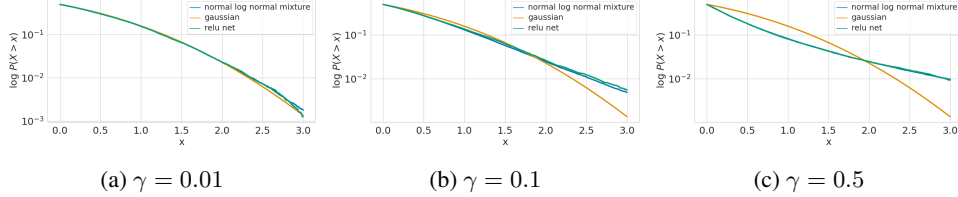
Figure 2: Convergence to normal log-normal mixture: We display the CDFs of a ReLU network, standard Gaussian CDF and the normal log-normal mixture. The width is fixed to 100 while depth is increased from 1 to 50 using the parameter \gamma . The neural network CDF is constructed empirically by drawing 10^4 samples from the prior. Note that as depth increases, the CDF departs from the Gaussian but still follows the normal log-normal mixture.
