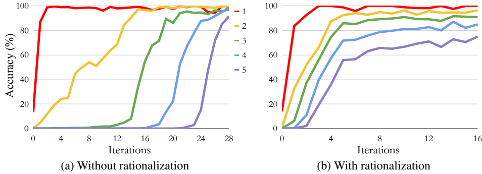
Figure 4: A visualization of the accuracy of n -digit summation with each iteration of STaR with and without rationalization. Each series corresponds to the accuracy of summing two n -digit numbers.
