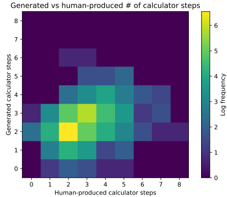
Figure 6: A comparison of the number of calculator steps generated by the model to solve examples in the training set relative to the number of steps used in the ground truth.
