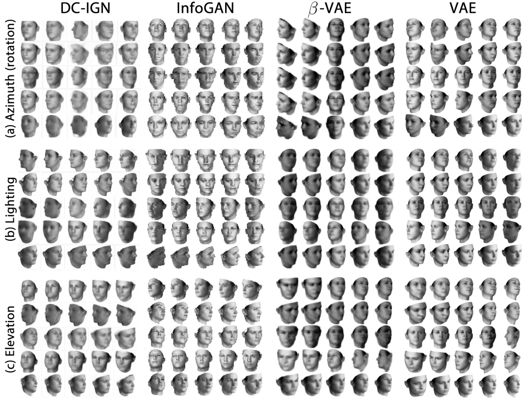
Figure 4: Manipulating latent variables on 3D faces: Qualitative results comparing disentangling performance of \beta -VAE ( \beta = 20 ), VAE (Kingma & Welling, 2014) ( \beta = 1 ), InfoGAN (Chen et al., 2016) and DC-IGN (Kulkarni et al., 2015). InfoGAN traversal is over the [-1, 1] range. All models learnt to disentangle lighting (b) and elevation (c). DC-IGN and VAE struggled to continuously interpolate between different azimuth angles (a), unlike \beta -VAE, which additionally learnt to encode a wider range of azimuth angles than other models. InfoGAN and DC-IGN images adapted from Chen et al. (2016) and Kulkarni et al. (2015), respectively. Reprinted with permission.
