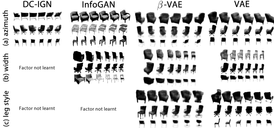
Figure 3: Manipulating latent variables on 3D chairs: Qualitative results comparing disentangling performance of \beta -VAE ( \beta = 5 ), VAE (Kingma & Welling, 2014) ( \beta = 1 ), InfoGAN (Chen et al., 2016) and DC-IGN (Kulkarni et al., 2015). InfoGAN traversal is over the [-1, 1] range. VAE always learns an entangled representation (e.g. chair width is entangled with azimuth and leg style (b)). All models apart from VAE learnt to disentangle the labelled data generative factor, azimuth (a). InfoGAN and \beta -VAE were also able to discover unlabelled factors in the dataset, such as chair width (b). Only \beta -VAE, however, learnt about the unlabelled factor of chair leg style (c). InfoGAN and DC-IGN images adapted from Chen et al. (2016) and Kulkarni et al. (2015), respectively. Reprinted with permission.
