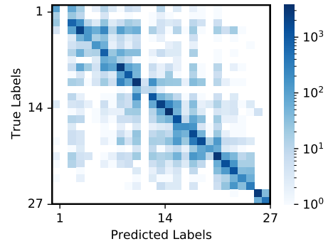
(a) Log-scale Confusion Matrix
