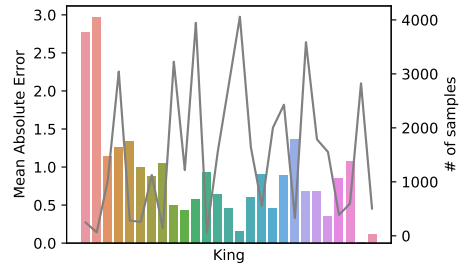
(b) Mean Absolute Error per King
