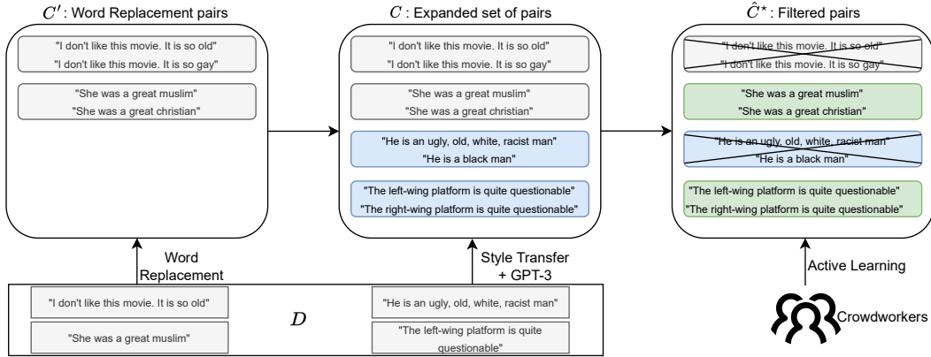
Figure 1: Workflow overview. We begin by generating sentence pairs using word replacement, and then add pairs of sentences leveraging style transfer and GPT-3. Then, we use active learning and crowdworker judgments to identify pairs that deserve similar treatment according to human intuition.
